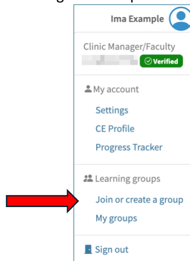
Figure 1. Drop-down Menu
